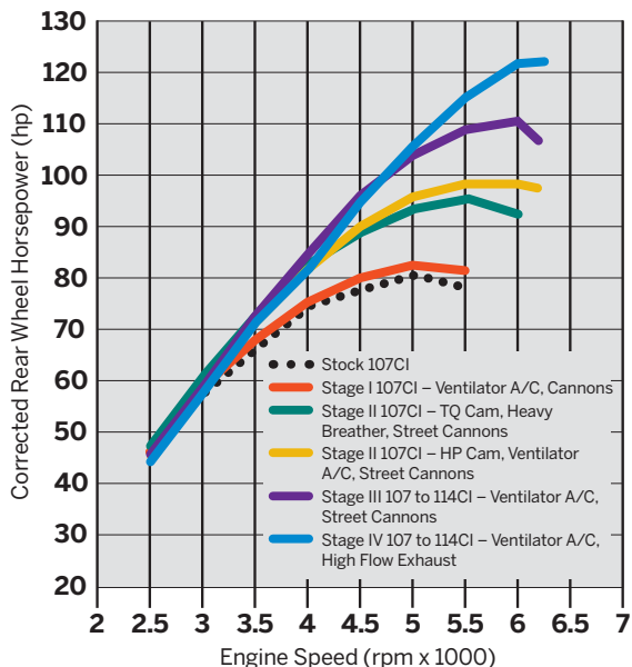
Milwaukee-Eight 107 Touring Stage Kits—Horsepower Comparisons
