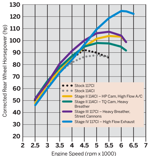
CVO Touring Stage Kits—Horsepower Comparisons
