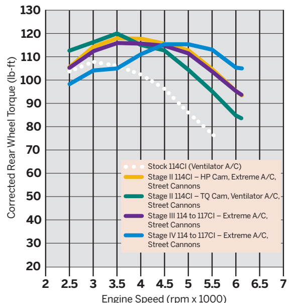
Milwaukee-Eight 114 Softail Stage Kits—Torque Comparisons
