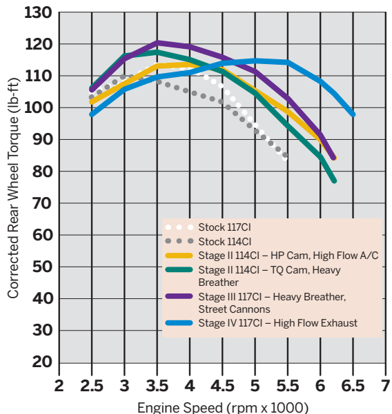
CVO Touring Stage Kits—Torque Comparisons
