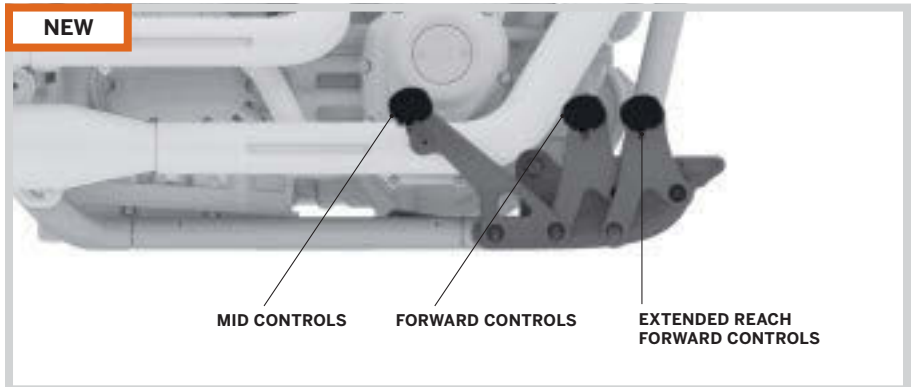
D. EXTENDED REACH FORWARD CONTROL KIT
