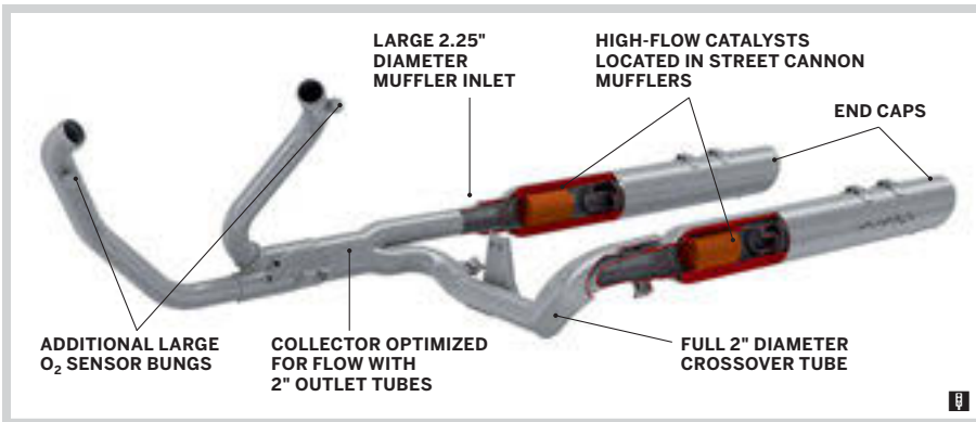
F. SCREAMIN' EAGLE HIGH-FLOW EXHAUST SYSTEM WITH STREET CANNON MUFFLERS
