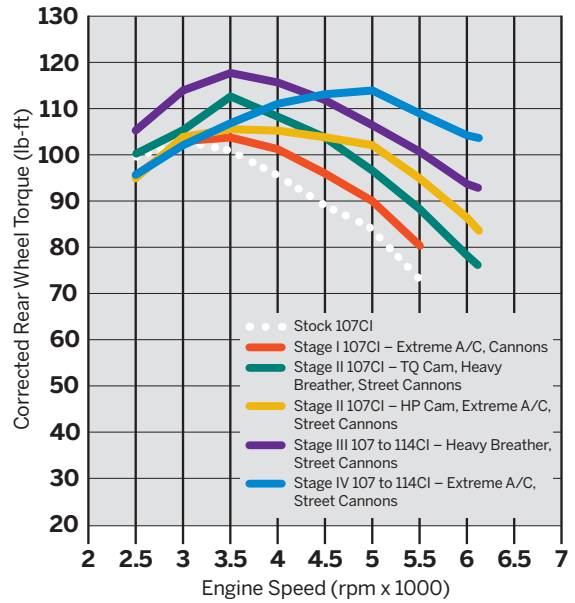
Milwaukee-Eight 107 Softail Stage Kits—Torque Comparisons
