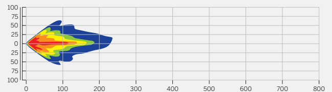
Projector LED Headlamp Low Beam (7'') Birds Eye View (shown in feet)
